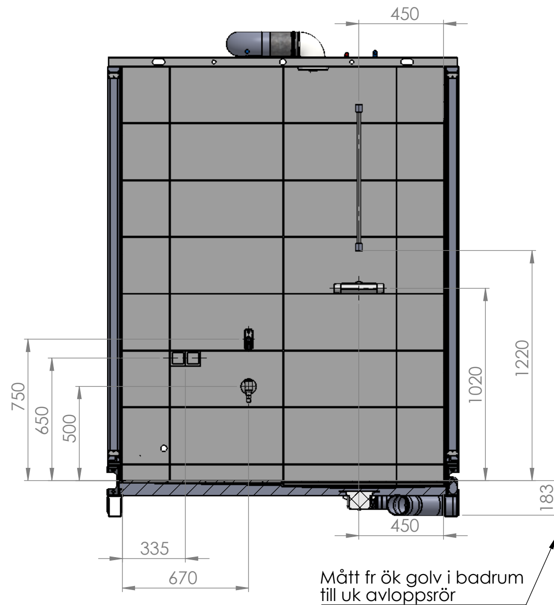
SECTION M-M SCALE 1 : 20
